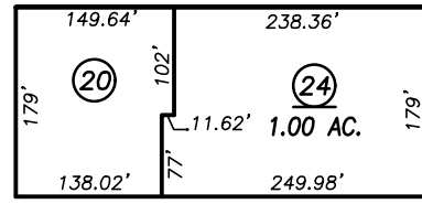
DETAIL 1 1"=200'
